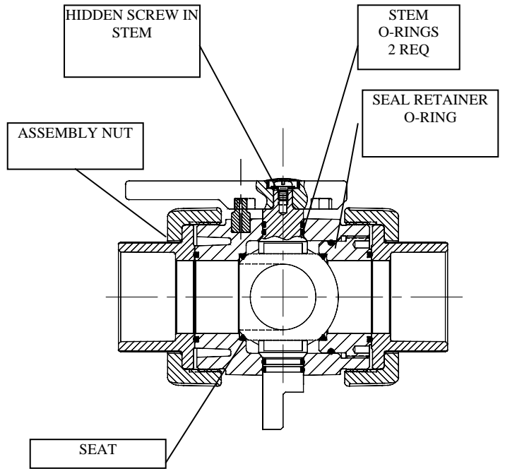
VALVE ILLUSTRATED
